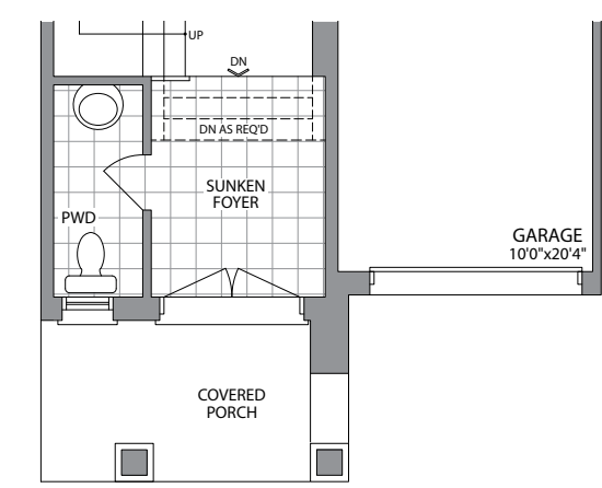
GROUND FLOOR ELEVATION 2
