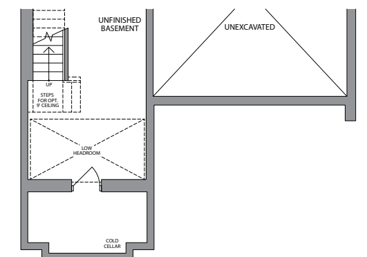
BASEMENT ELEVATION 2
