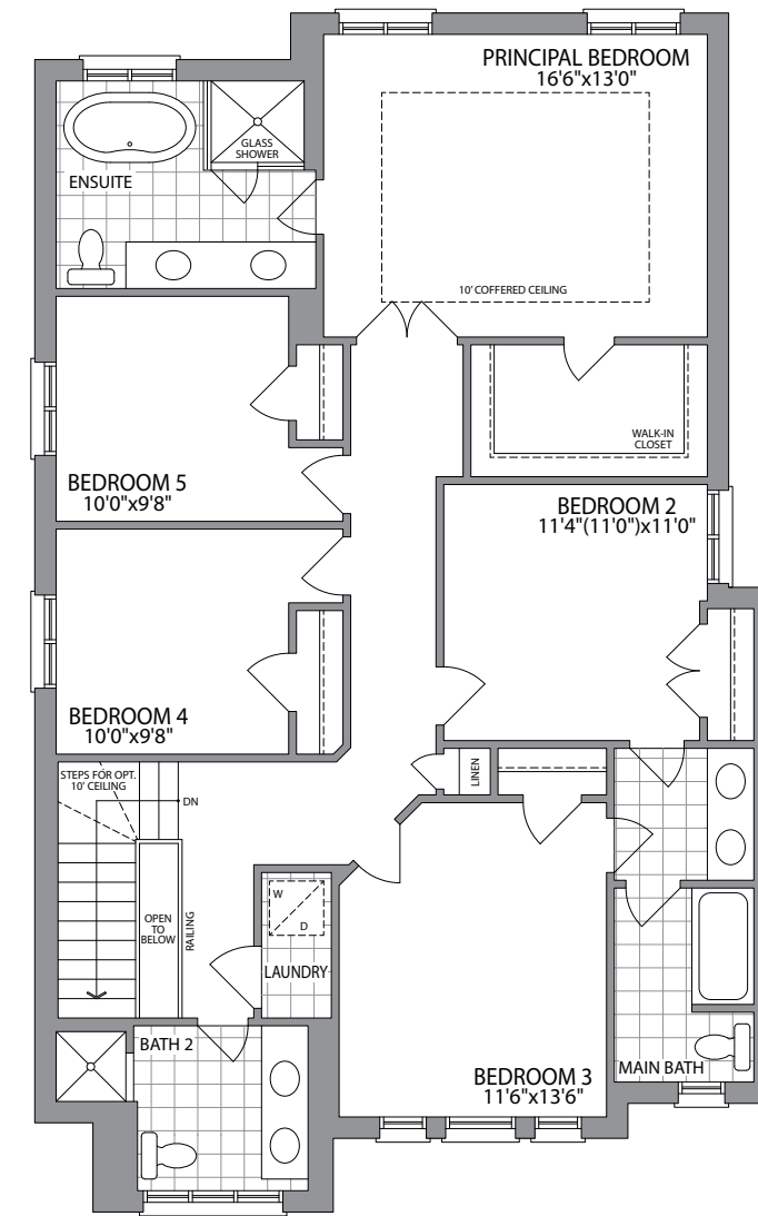
OPT. SECOND FLOOR W/5 BEDROOMS ELEVATION 1
