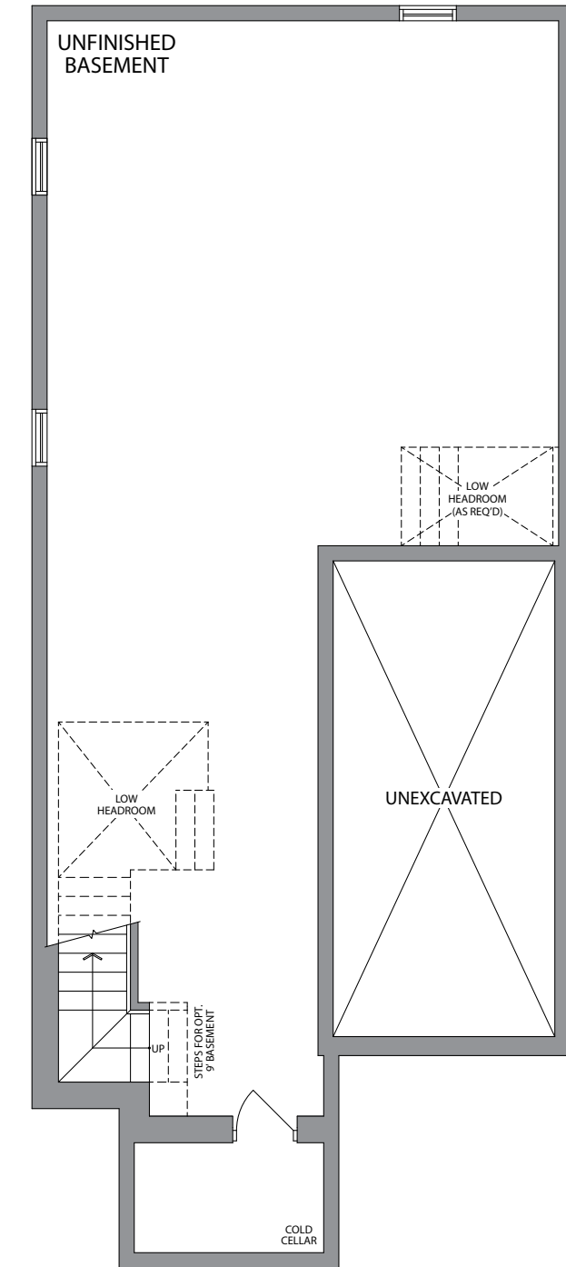
BASEMENT ELEVATION 1 & 2
