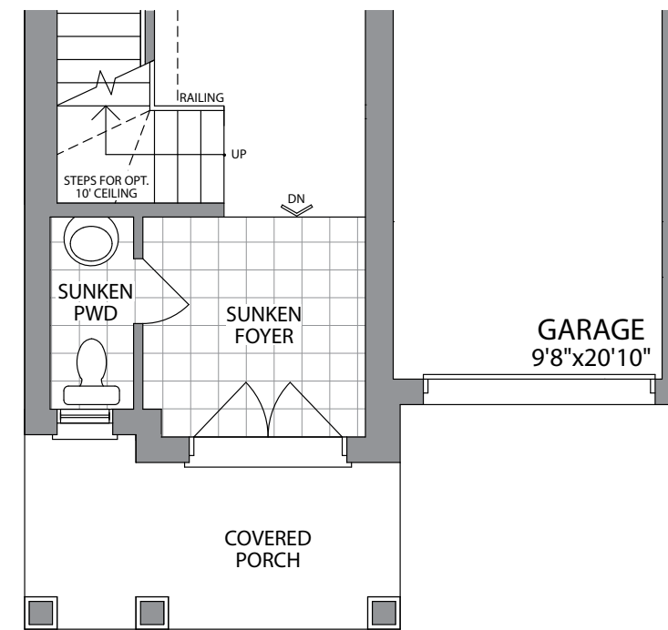
GROUND FLOOR ELEVATION 2
