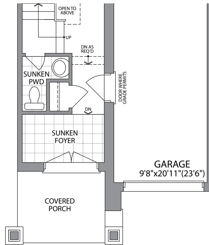
GROUND FLOOR ELEVATION 2
