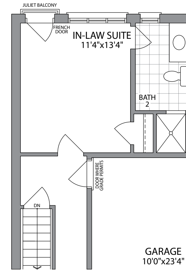
OPT. GROUND FLOOR W/IN-LAW SUITE ELEVATION 1C & 2C
