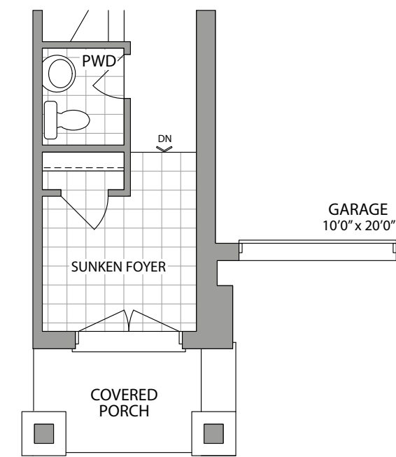
GROUND FLOOR ELEVATION 2
