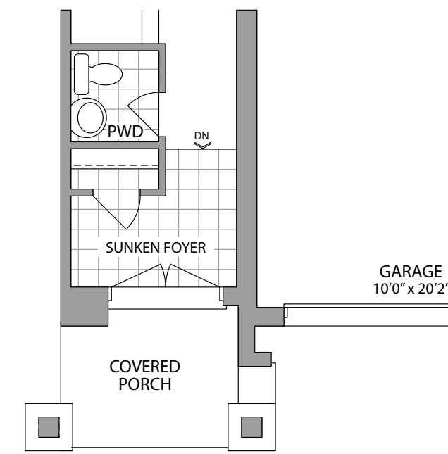
GROUND FLOOR ELEVATION 2
