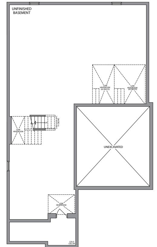
BASEMENT ELEVATION 1
