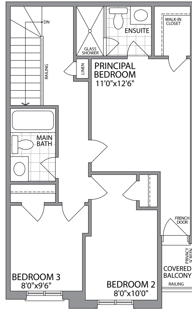
THIRD FLOOR ELEVATION 1 & 2
