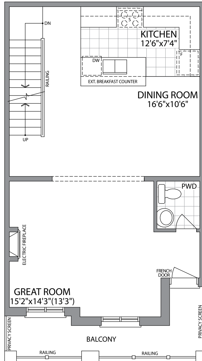
MAIN FLOOR ELEVATION 1
