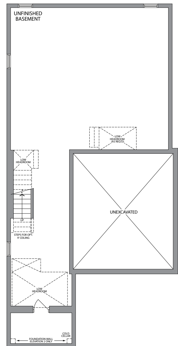
BASEMENT ELEVATION 1 & 2
