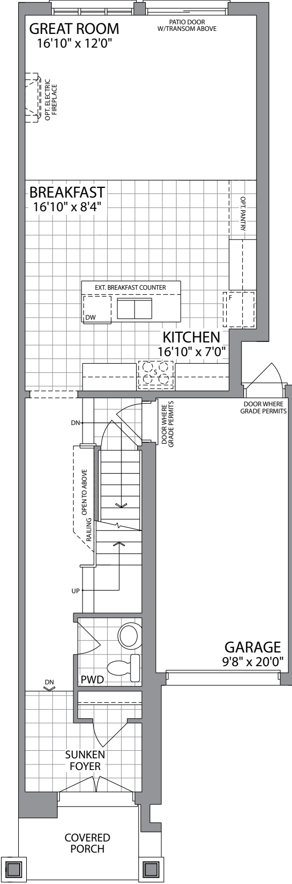
GROUND FLOOR ELEVATION 1 & 2
