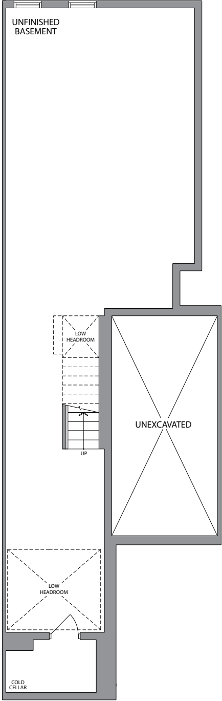
BASEMENT ELEVATION 1 & 2
