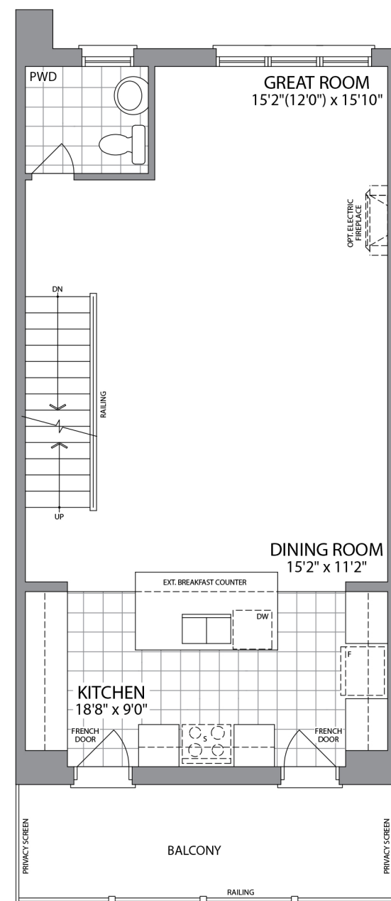
MAIN FLOOR ELEVATION 1
