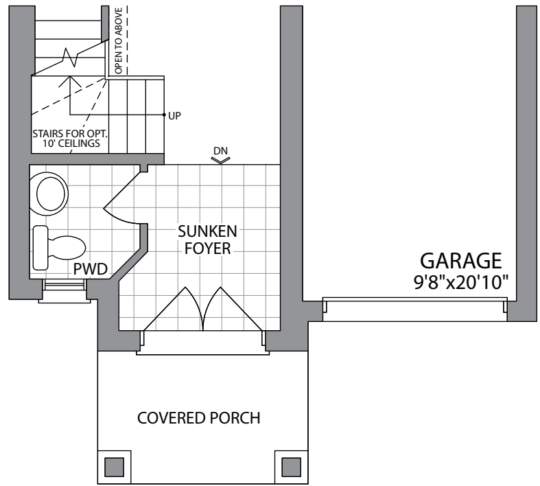
GROUND FLOOR ELEVATION 2
