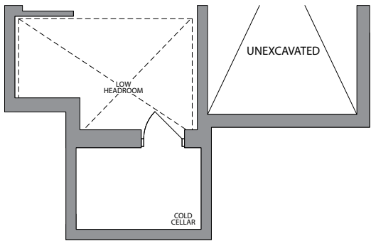
BASEMENT ELEVATION 2
