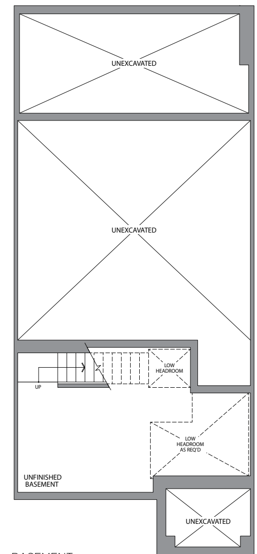
BASEMENT ELEVATION 1
