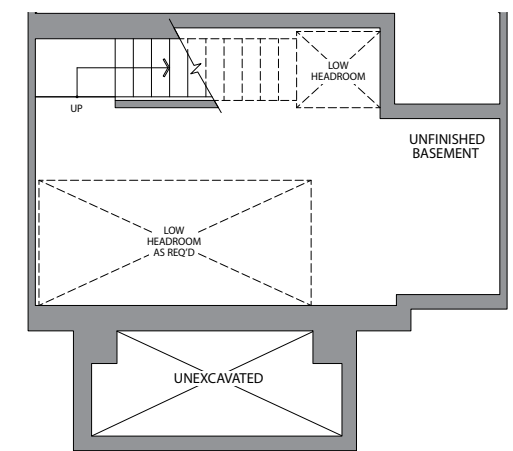
BASEMENT ELEVATION 2
