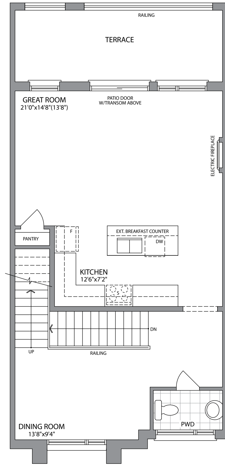
MAIN FLOOR ELEVATION 1
