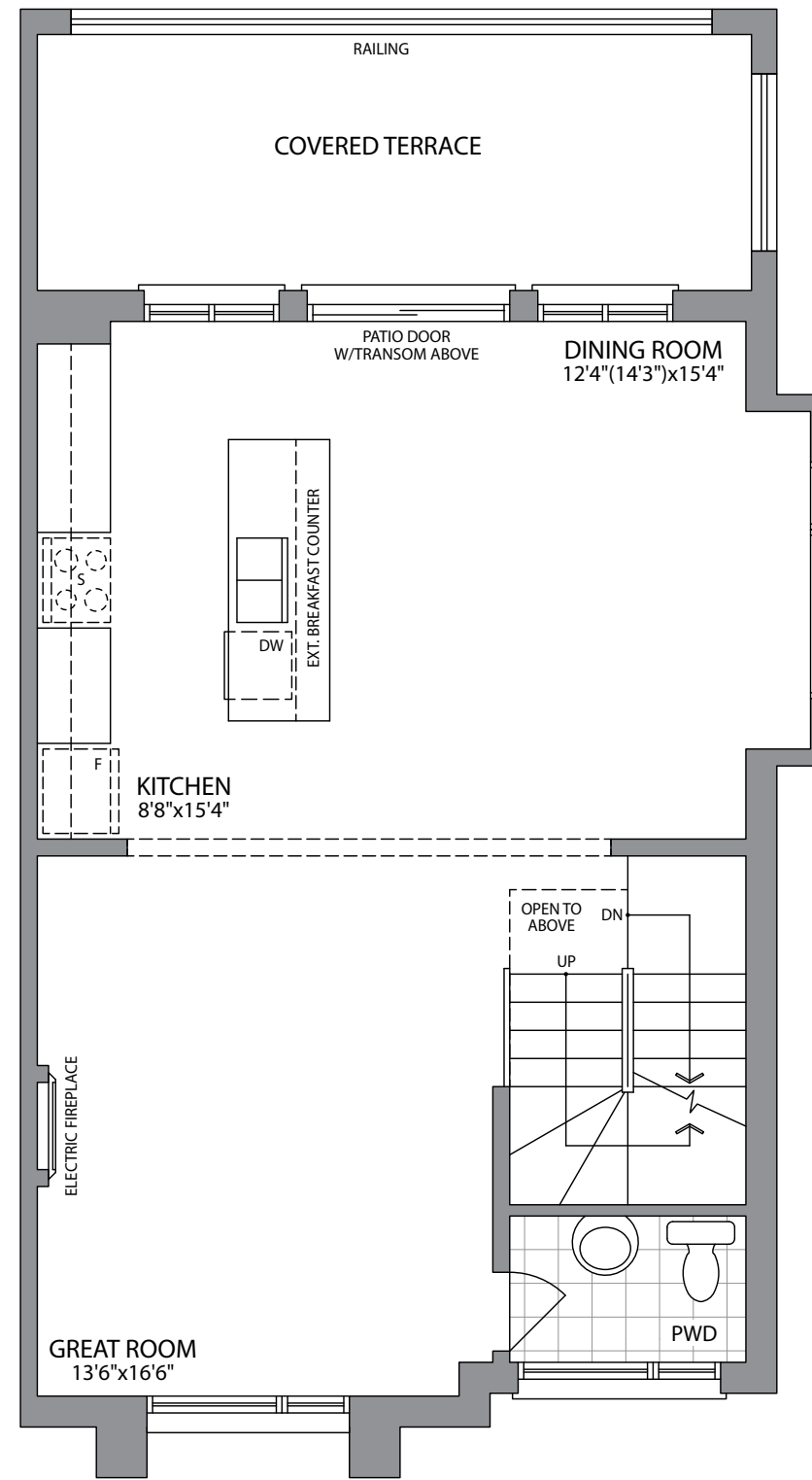
MAIN FLOOR ELEVATION 1C
