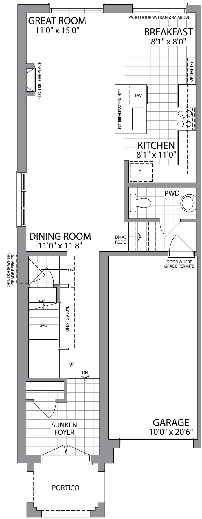
GROUND FLOOR ELEVATION 1 & 2
