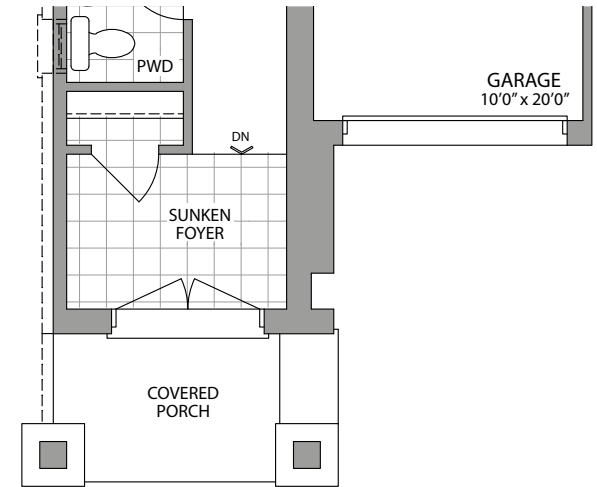
GROUND FLOOR ELEVATION 2/2C
