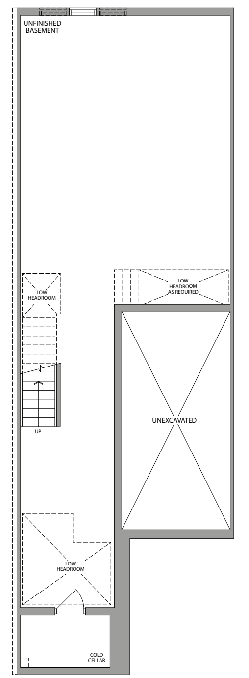
BASEMENT ELEVATION 1/1C & 2/2C
