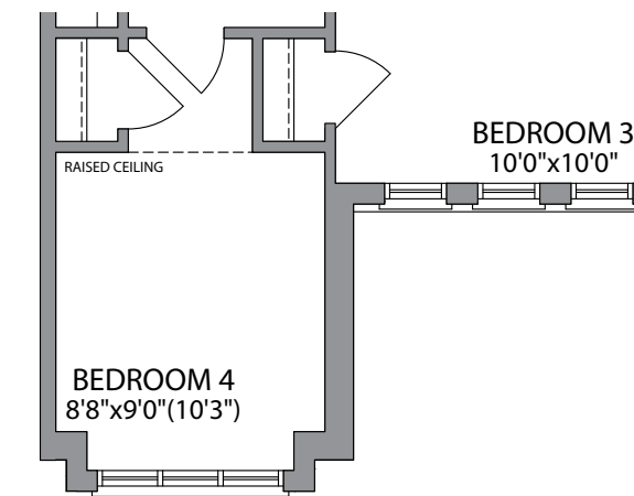
SECOND FLOOR ELEVATION 2
