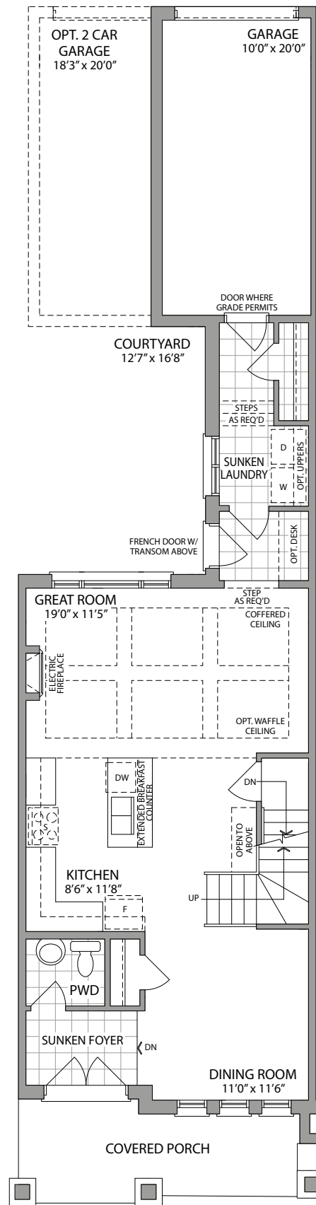
GROUND FLOOR ELEVATION 1
