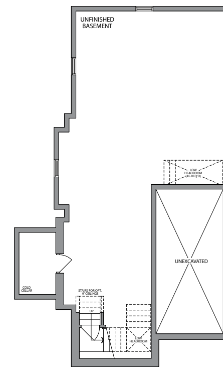
BASEMENT ELEVATION 1C
