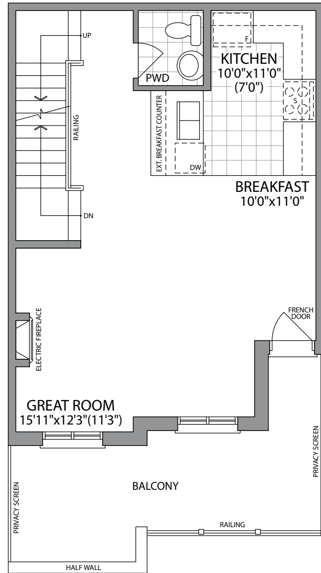
THIRD FLOOR ELEVATION 1
