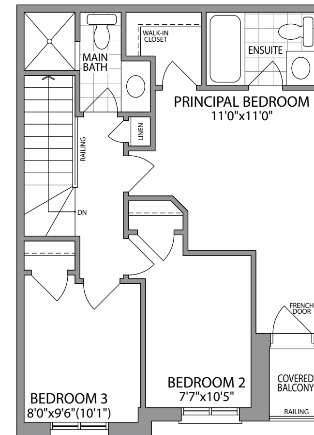
OPT. THIRD FLOOR W/EXTRA BATH ELEVATION 1
