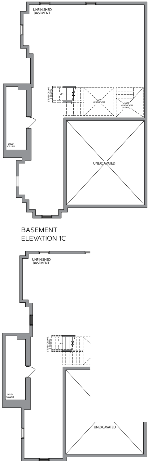
BASEMENT ELEVATION 2C
