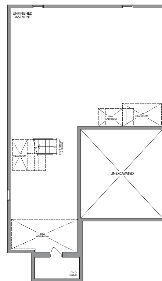
BASEMENT ELEVATION 1
