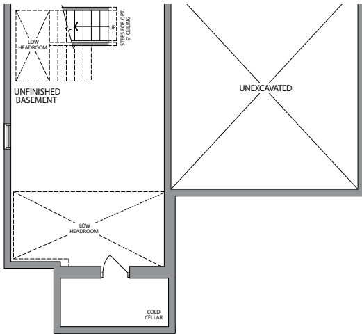
BASEMENT ELEVATION 2
